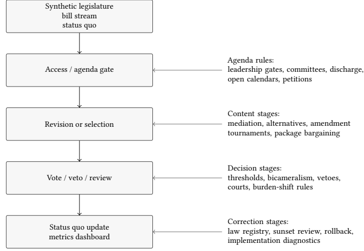
Fig. 1. Modular simulation pipeline. Each institutional bundle intervenes at one or more stages while generated legislatures, bill streams, and status-quo-relative voting remain shared across comparisons.
