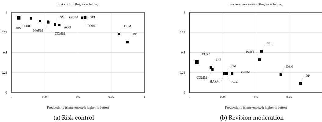
Fig. 2. Productivity tradeoff views for the representative systems. Panel (a) plots risk control across the main broad/adversarial campaign averages, with thin five-seed uncertainty bars where visible; panel (b) plots revision moderation under weighted party-system sensitivity cases. Higher is better on both y-axes. Labels are the mechanism-family labels from Table 3. The asterisk and larger square mark the stylized U.S.-like benchmark.
