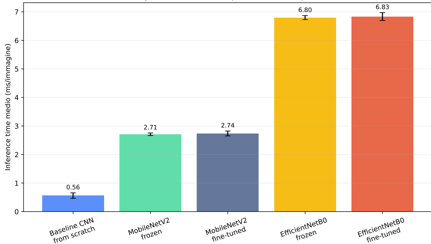
Model-only inference time comparison — k-fold patient-wise
