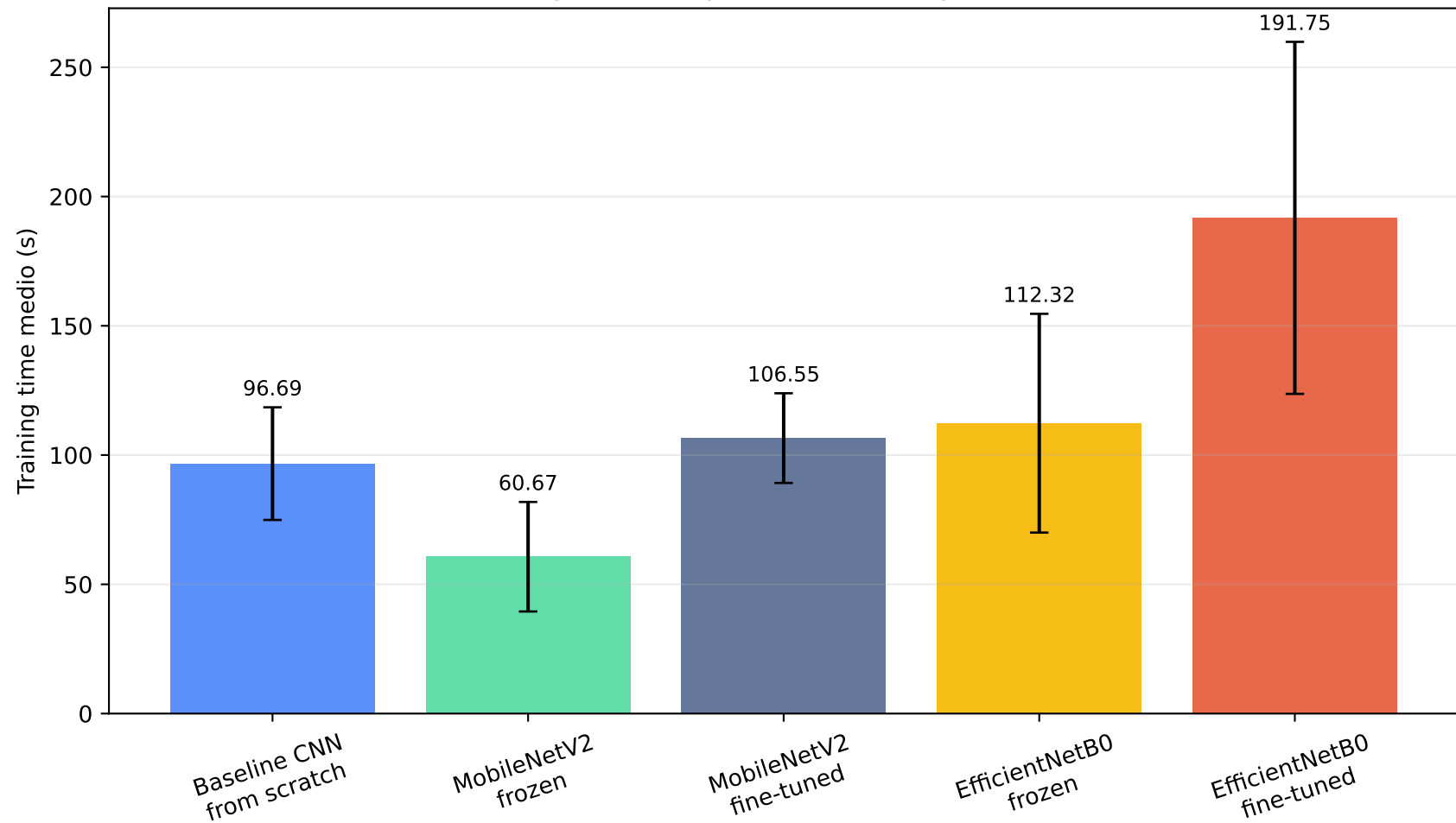
Training time comparison — k-fold patient-wise
