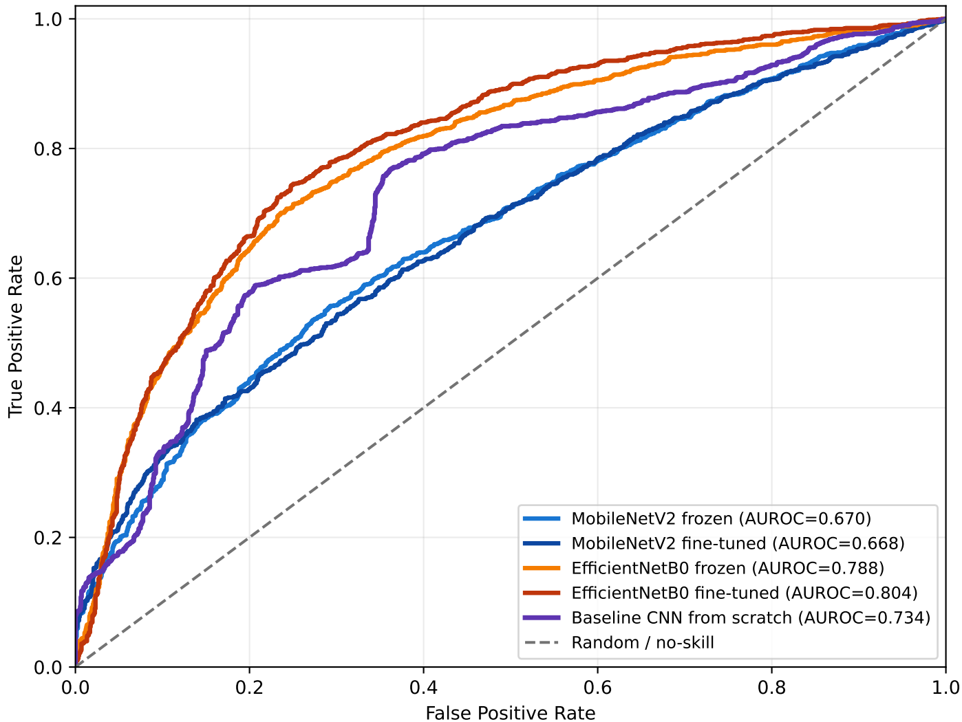
ROC curves — CNN baseline vs transfer learning
