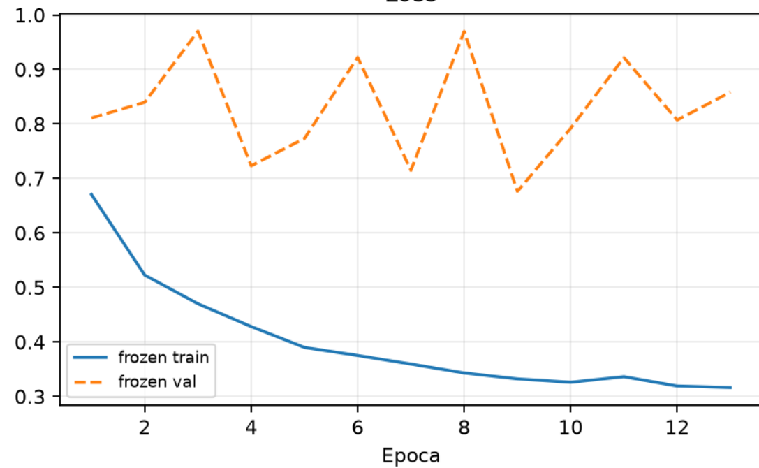
Loss
