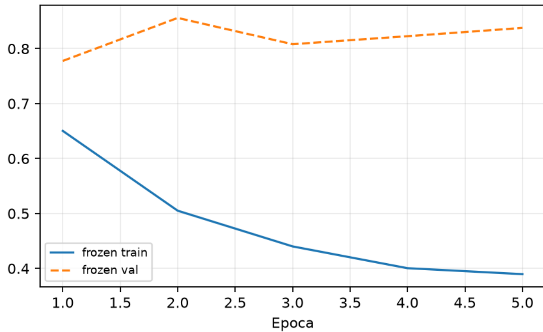
Loss
