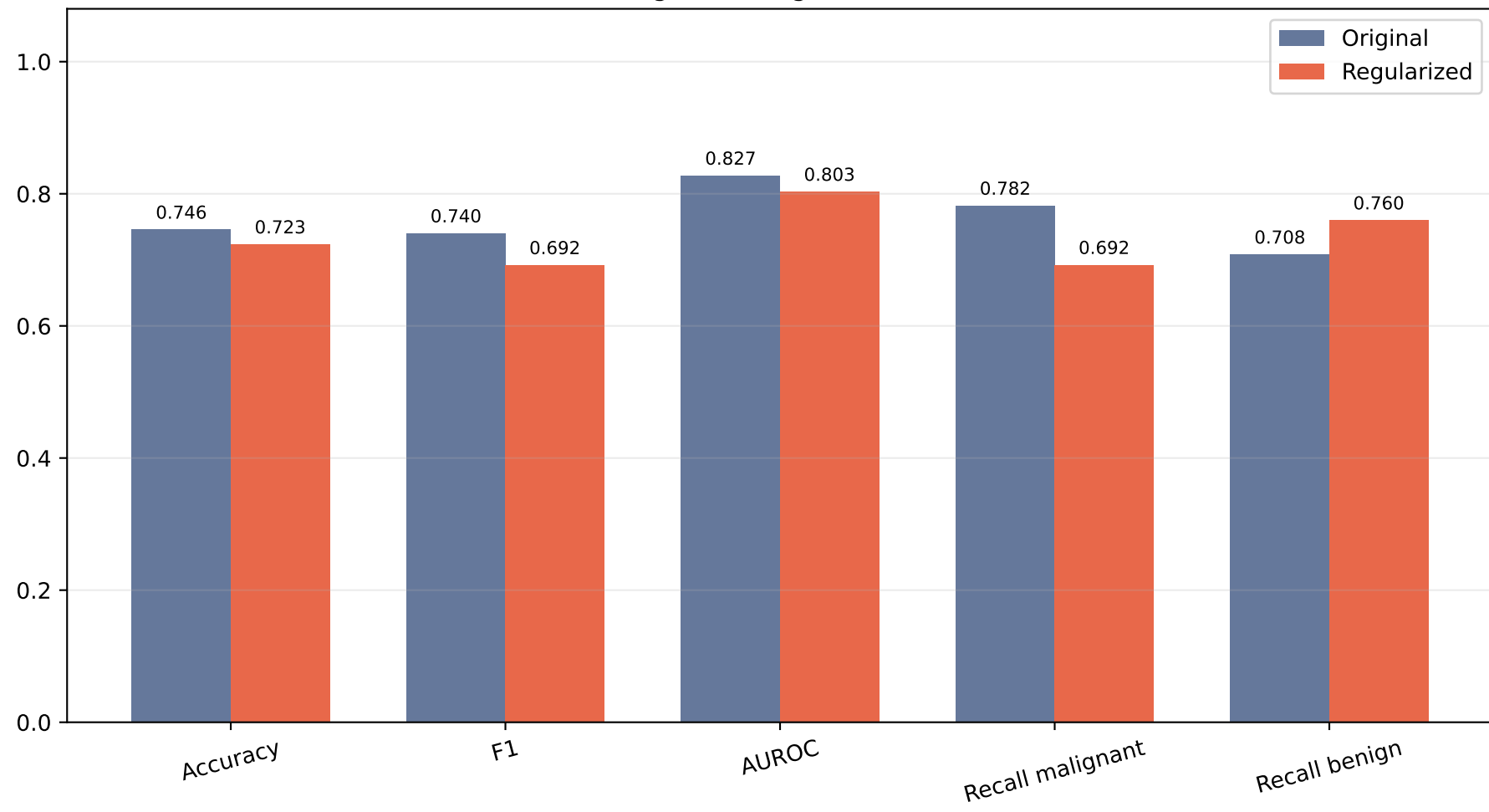
EfficientNetB0 original vs regularized — k-fold metrics
