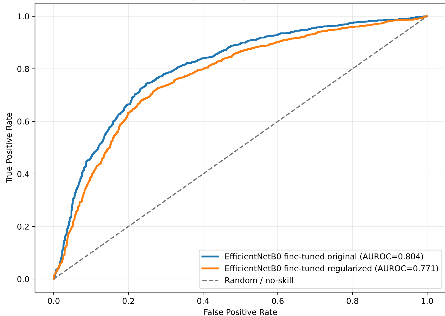
EfficientNetB0 original vs regularized ROC — out-of-fold
