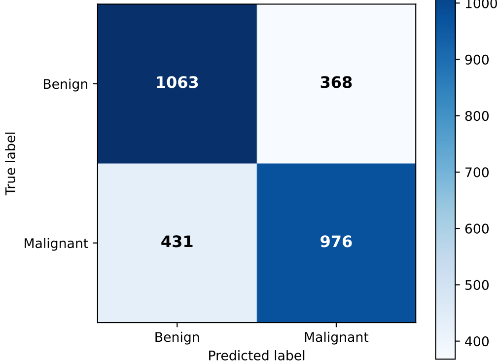
EfficientNetB0 fine-tuned regularized — aggregate out-of-fold
