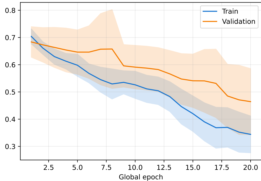
Loss
