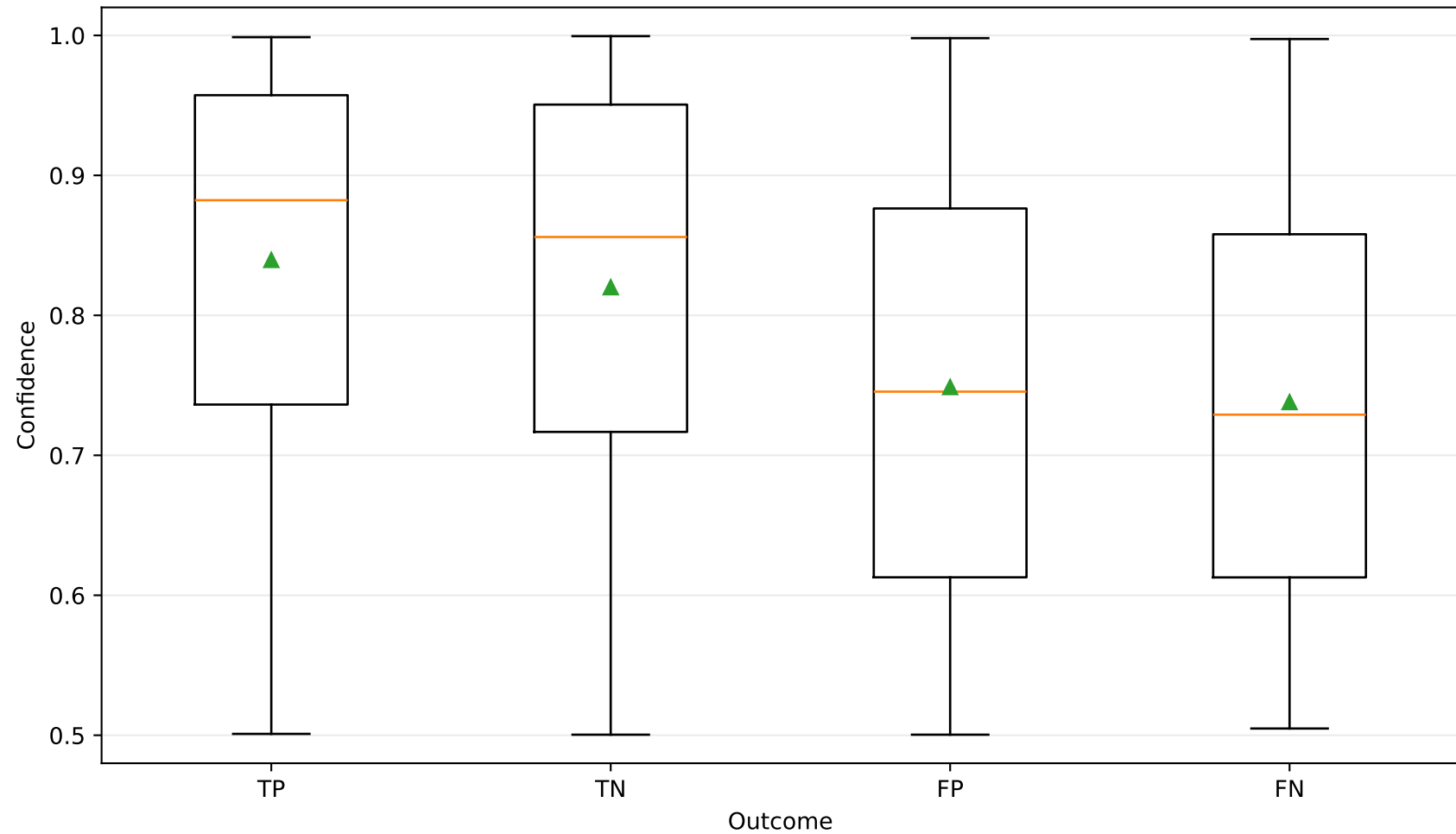
Confidence by prediction outcome
