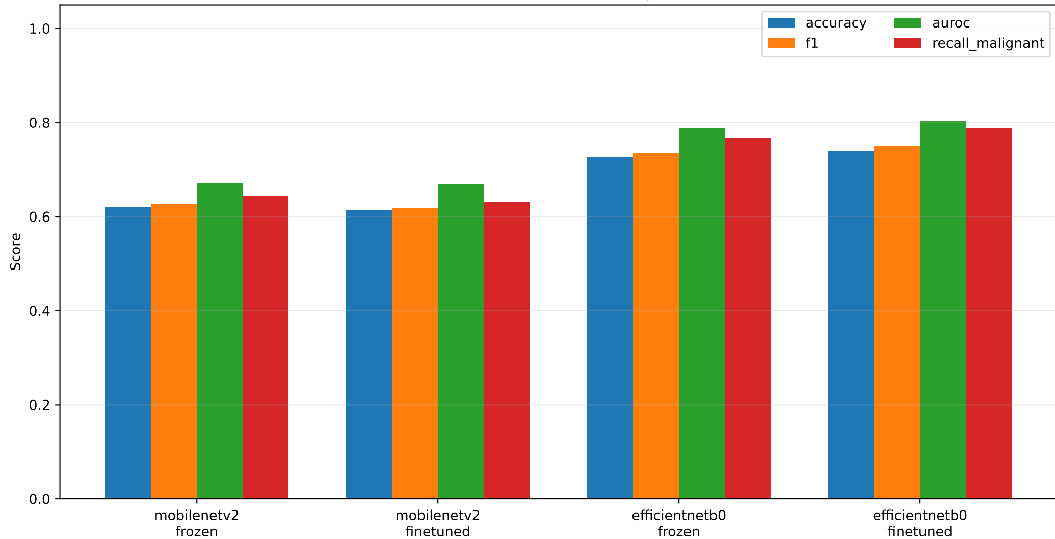
Overall out-of-fold transfer model performance
