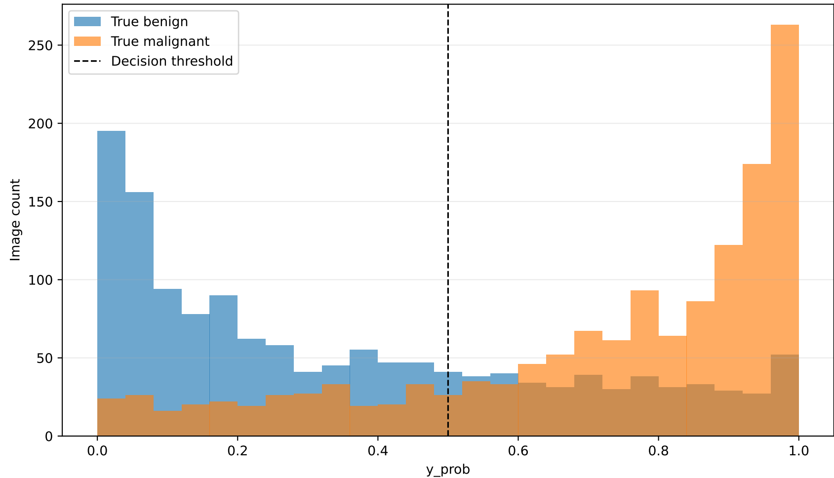
Predicted malignant probability by true class
