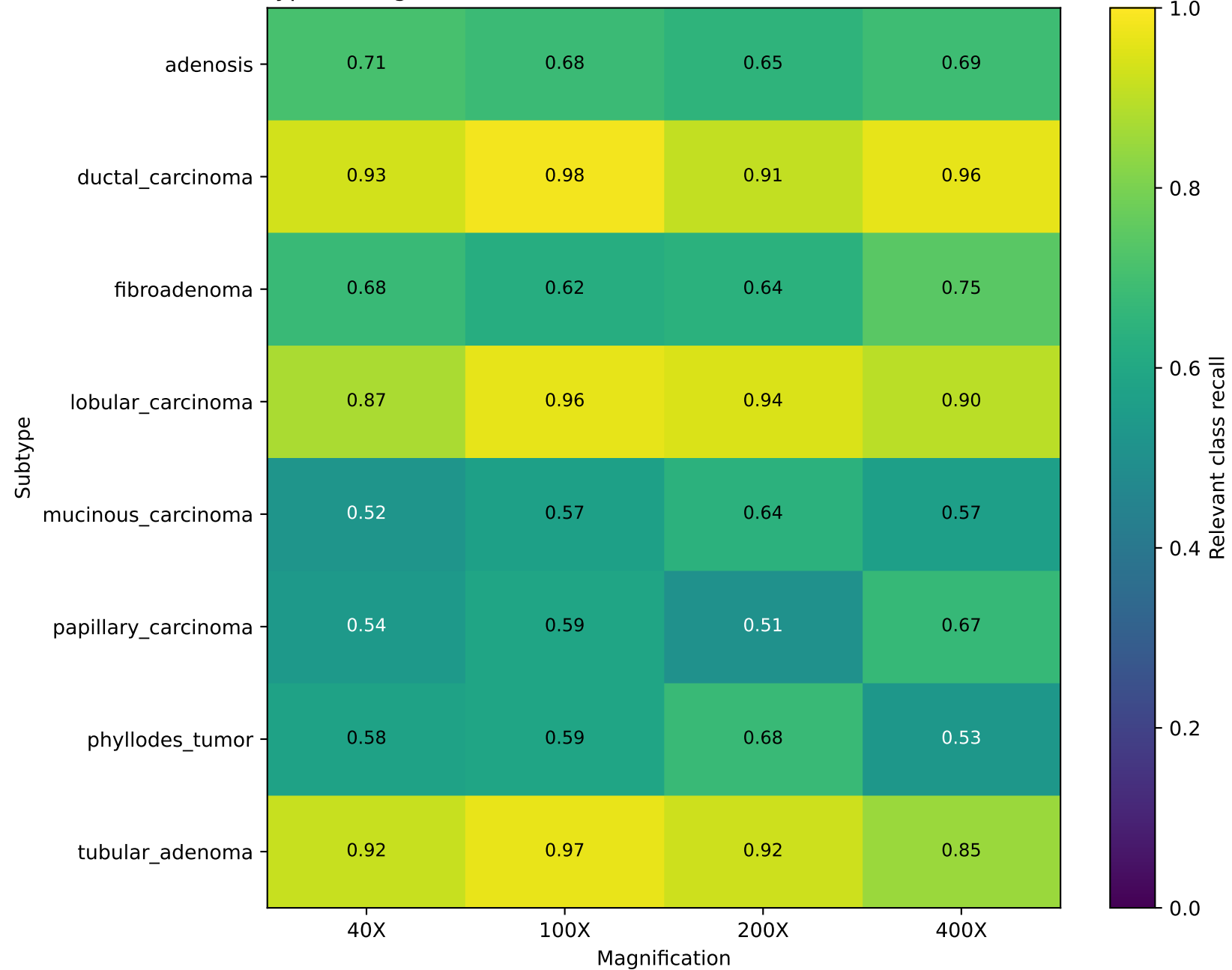
Subtype × magnification relevant class recall — EfficientNetB0 fine-tuned
