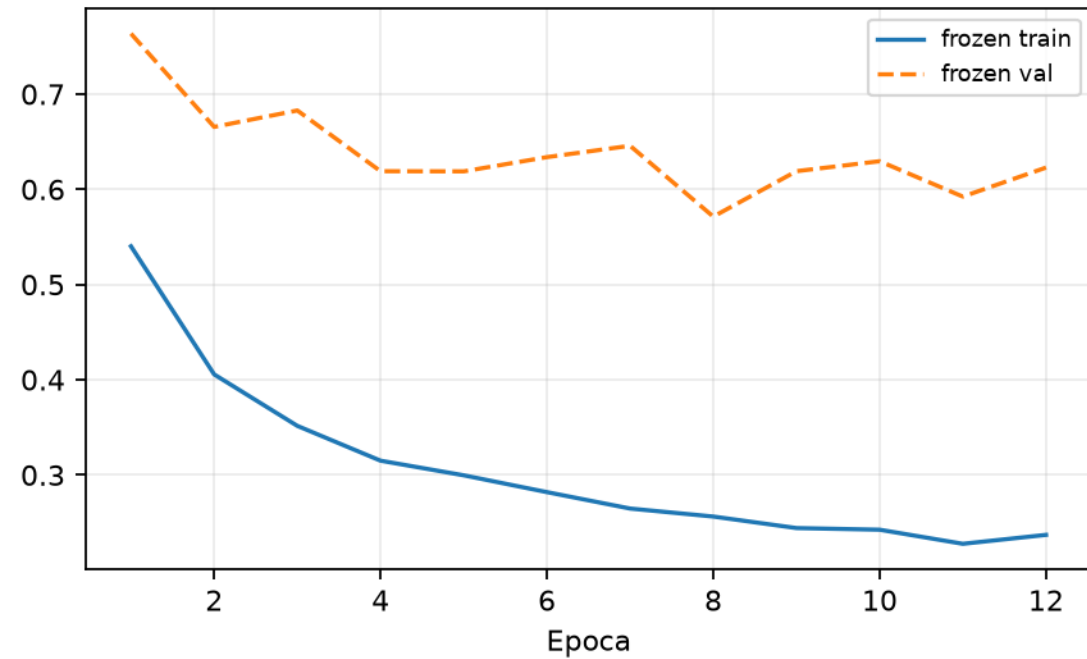
Loss
