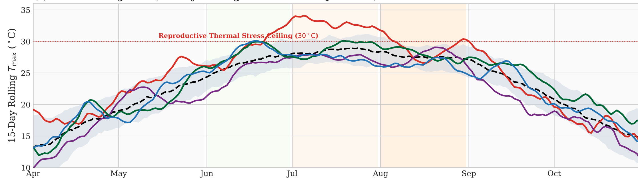
(c) Thermal Regimes (15-Day Rolling Maximum Temperature)
