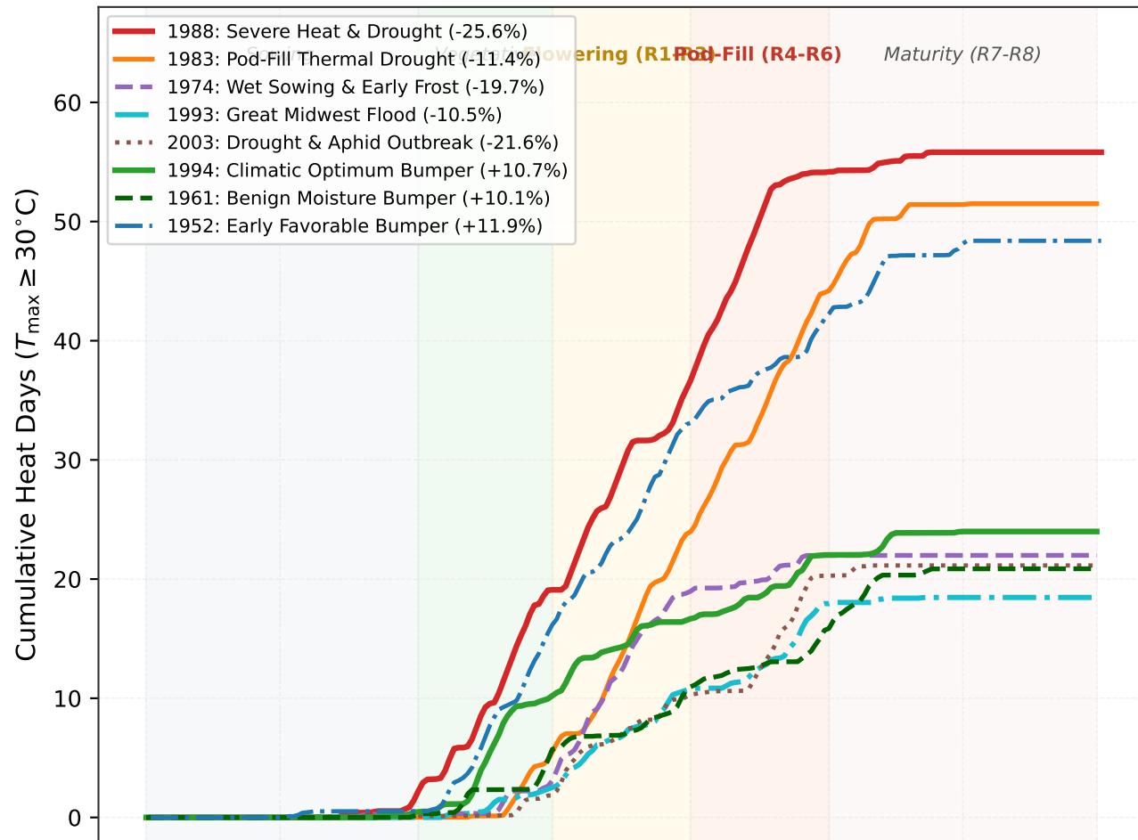
(a) Cumulative Extreme Heat Stress Exposure ( \sum HD_{30} )
