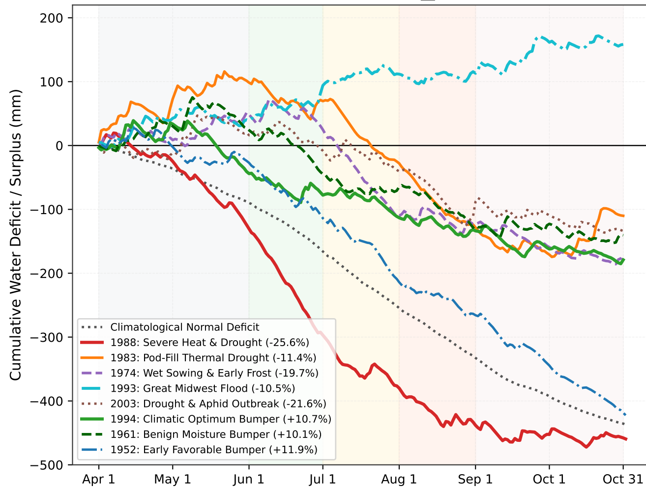
(c) Cumulative Climatic Water Budget ( \sum(P - ET_0) )
