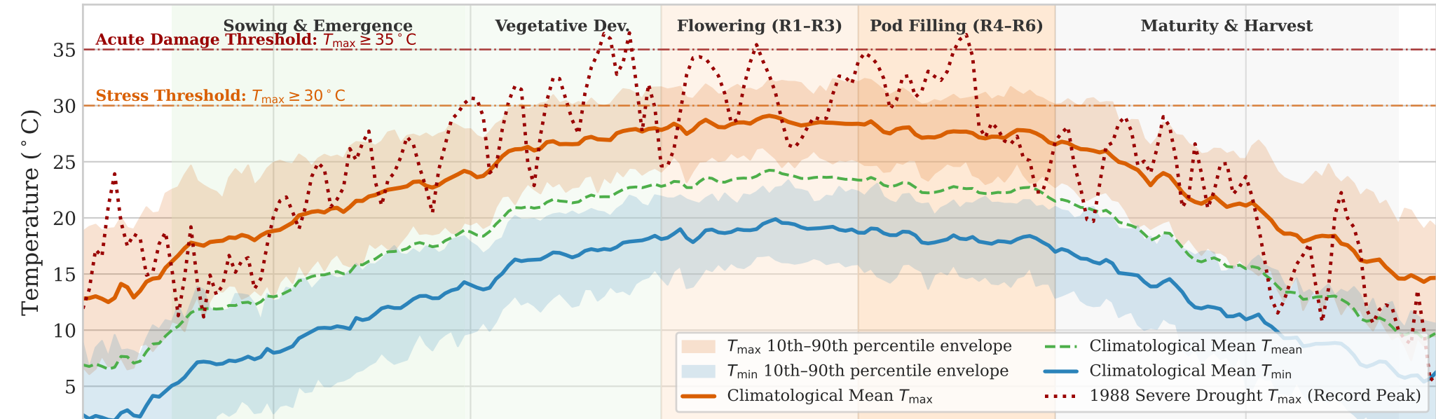
(a) Thermal Dynamics and Phenological Calendar Across the Growing Cycle (April 1 - October 31)
