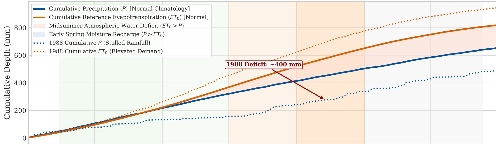
(b) Hydrological Budget: Cumulative Atmospheric Water Deficit ( P vs. ET_0 )
