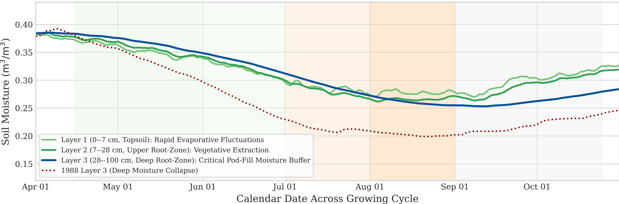
(c) Edaphic Moisture Depletion Across Rooting Horizons ( SM_1 , SM_2 , SM_3 )
