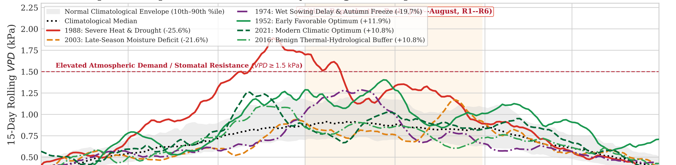
(a) Atmospheric Evaporative Demand: 15-Day Rolling Mean Vapor Pressure Deficit (VPD)
