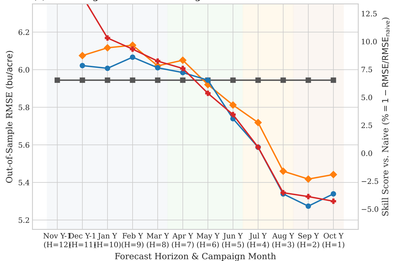
(b) Error Magnitude and Percentage Skill
