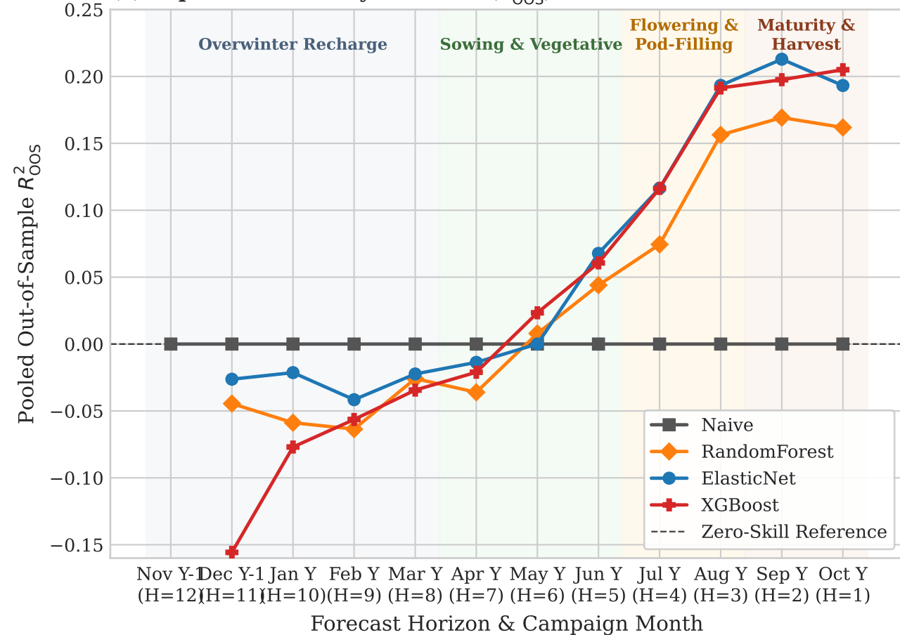
(a) Explained Anomaly Variance ( R^2_{\text{OoS}} )
