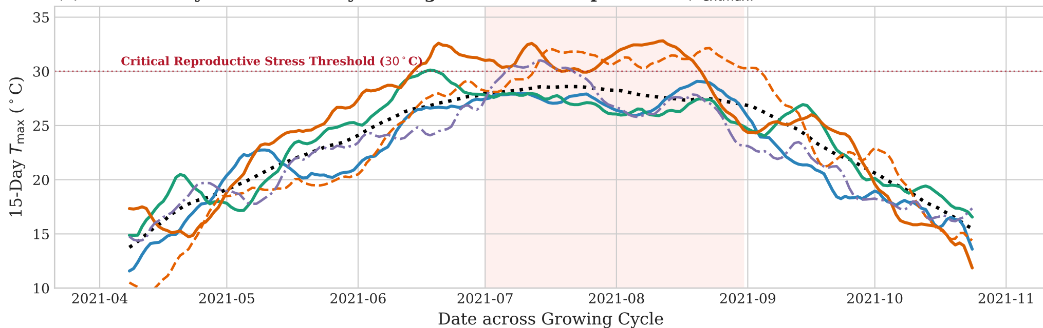
(c) Thermal Dynamics: 15-Day Rolling Maximum Temperature ( T_{\text{extmax}} )
