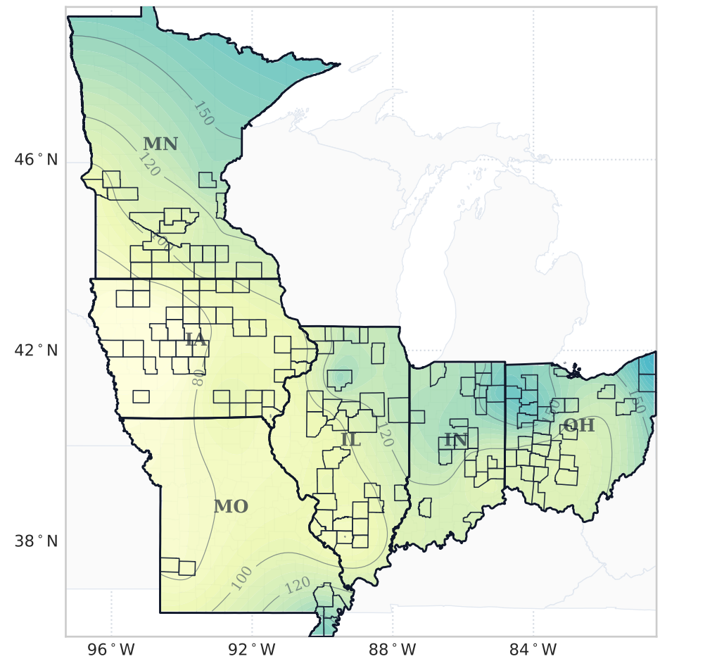
(a) 2012 Flash Drought: July-August Rainfall ( P )
