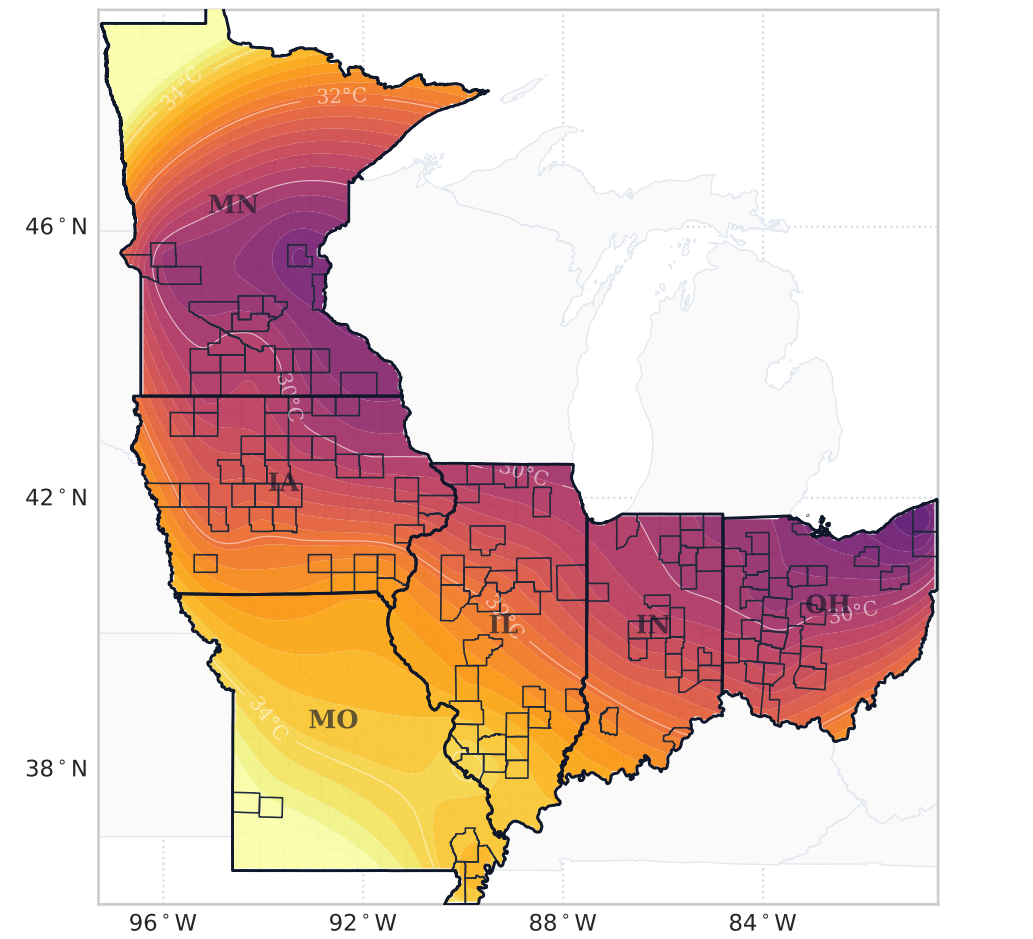
(b) 2012 Flash Drought: July-August Max Temp ( T_{\max} )
