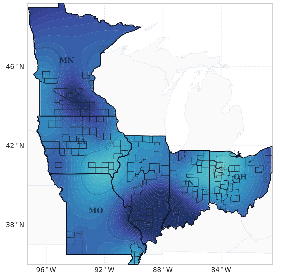
(c) 2016 Climatic Optimum: July-August Rainfall ( P )
