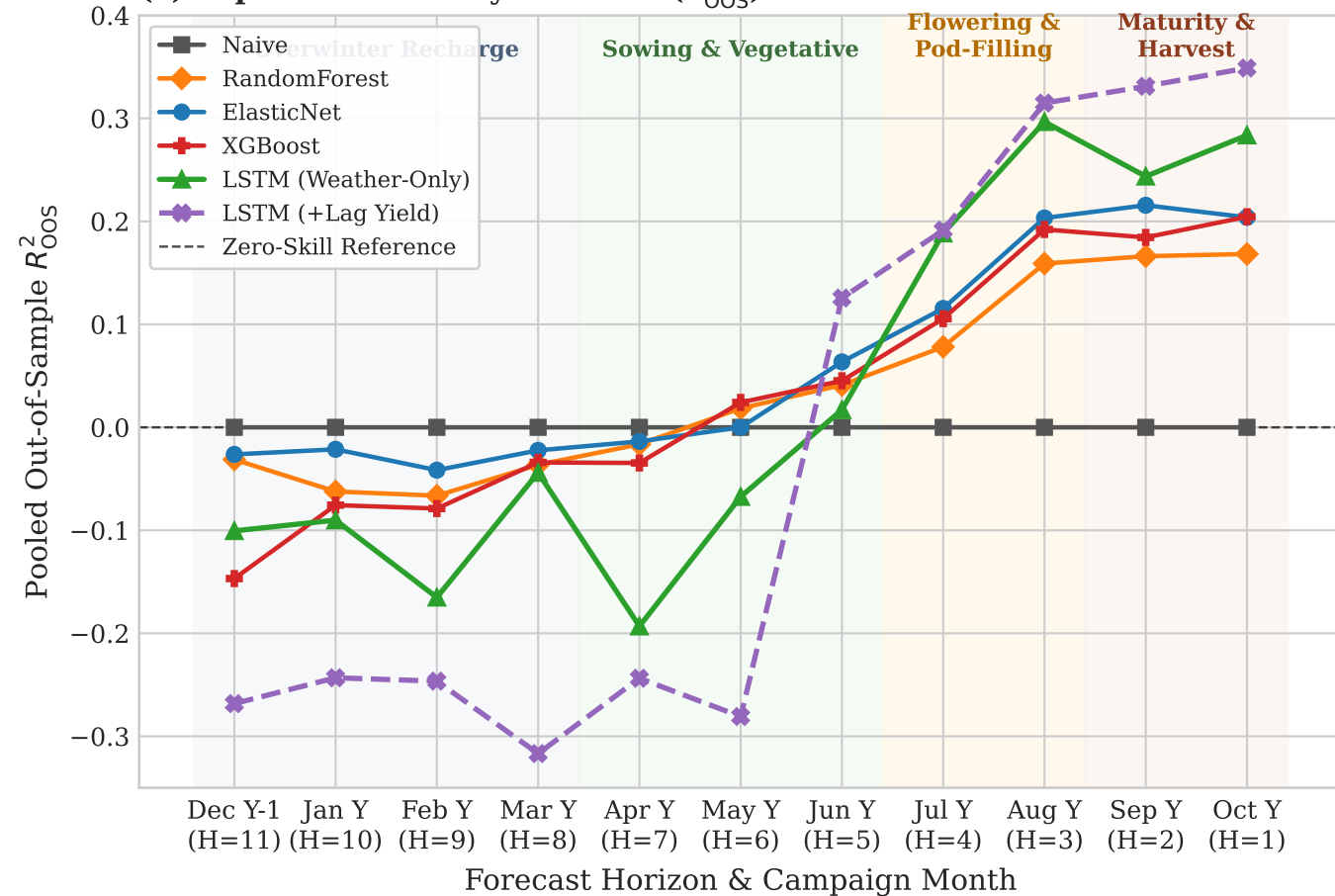
(a) Explained Anomaly Variance ( R^2_{00s} )
