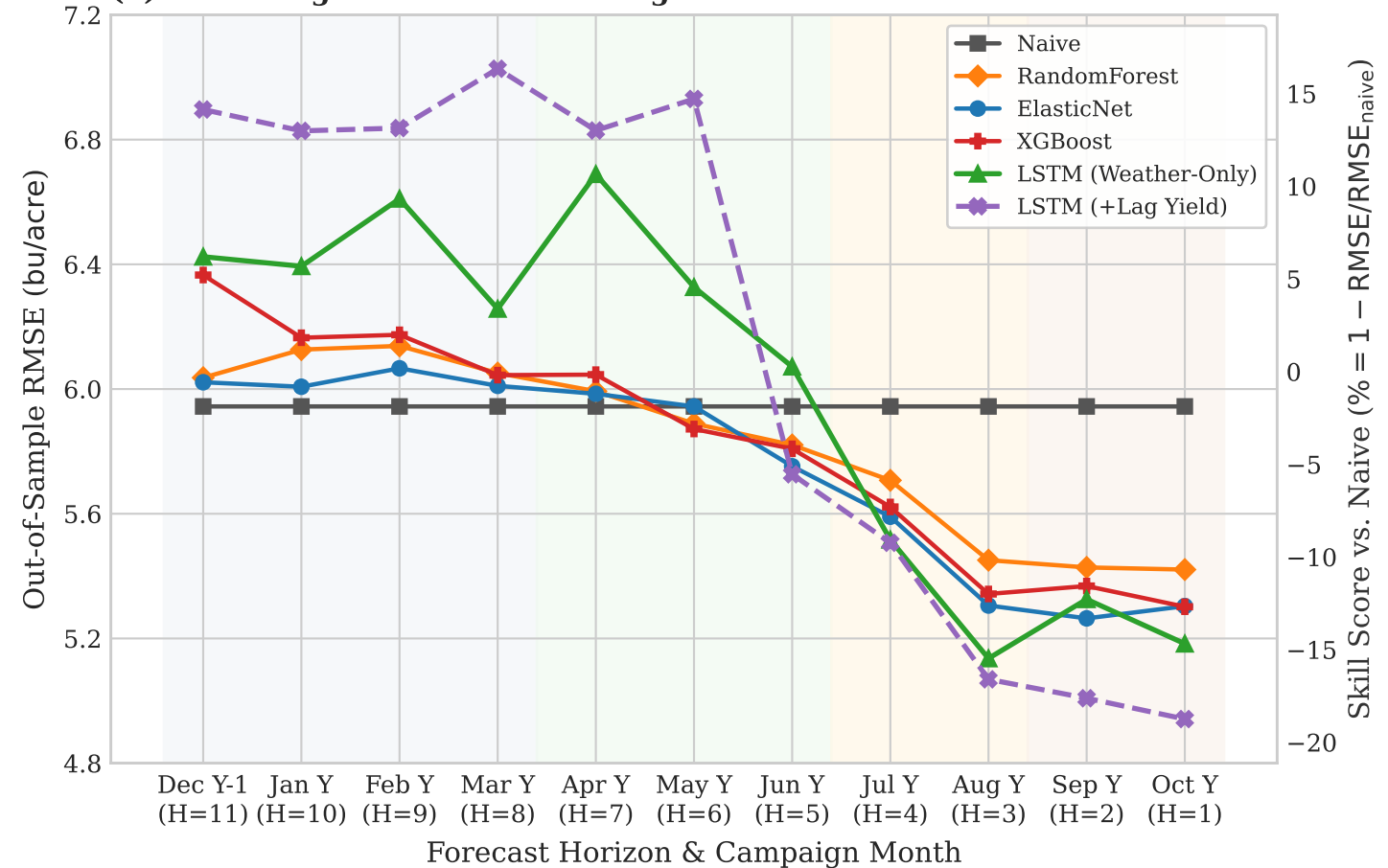
(b) Error Magnitude and Percentage Skill
