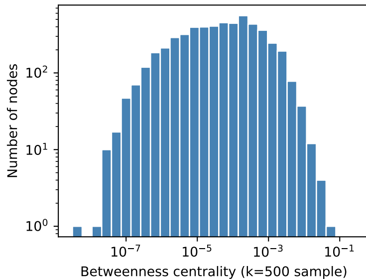
Degree-preserving randomized network
