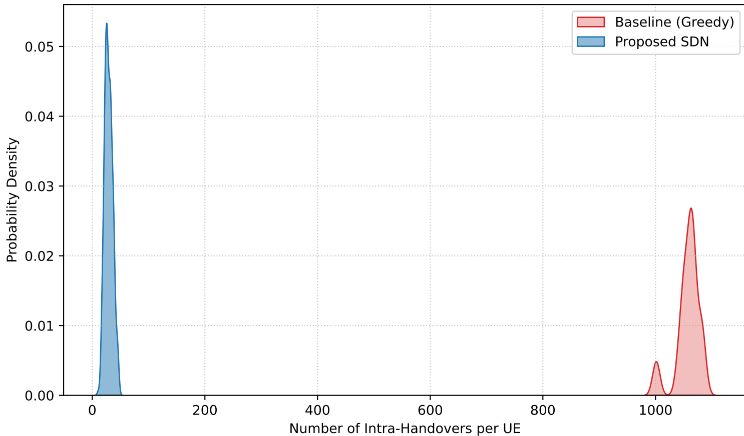
Intra-Satellite Handover Rate Comparison
