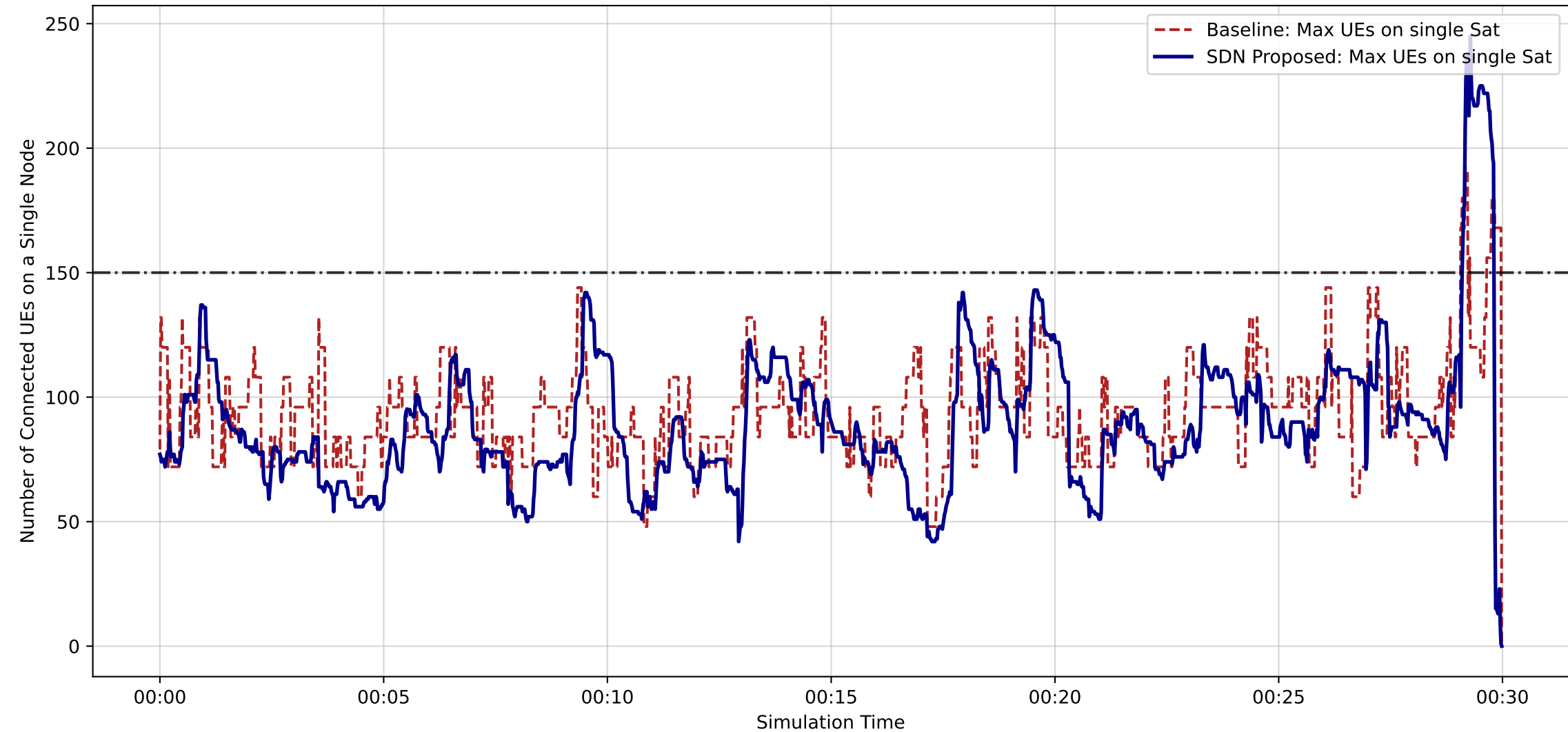
Network Congestion: Maximum Load per Satellite Comparison
