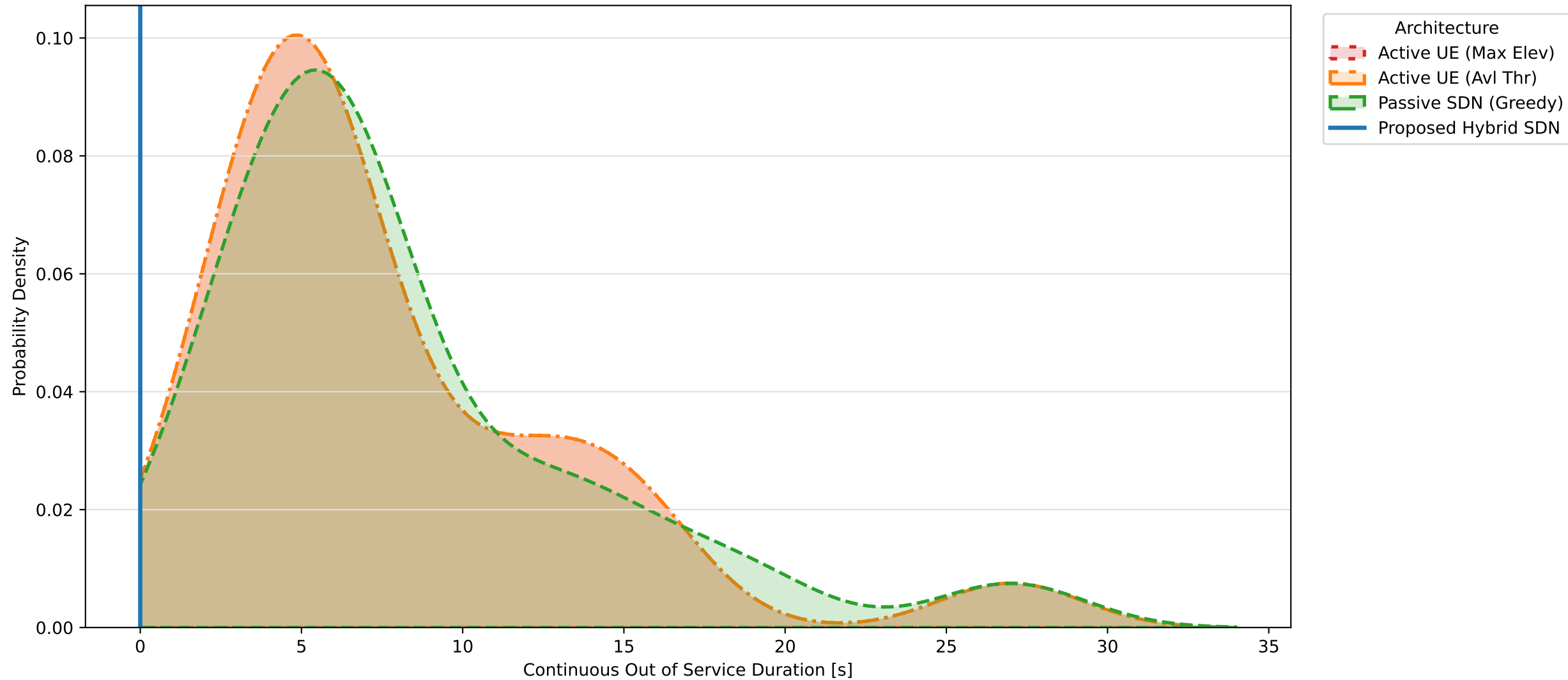
Probability Density of Out of Service (OOS) Time - 4-Way Comparison
