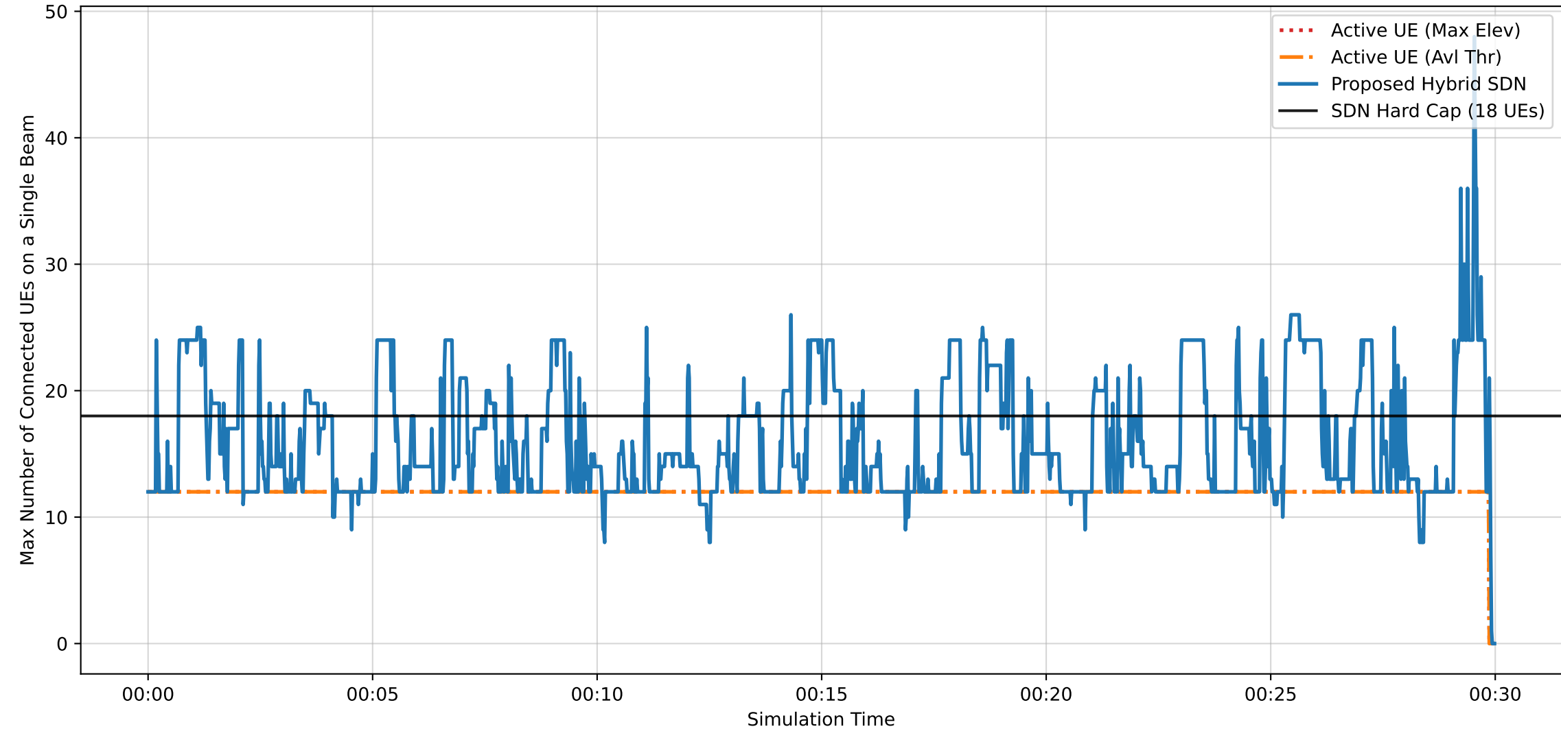
Network Congestion: Maximum Load on a Single Beam Comparison
