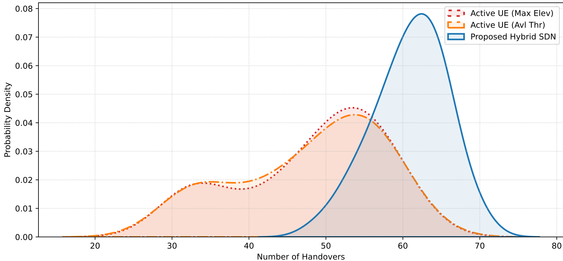
PDF of Inter-Satellite Handovers per UE - Comparative Analysis
