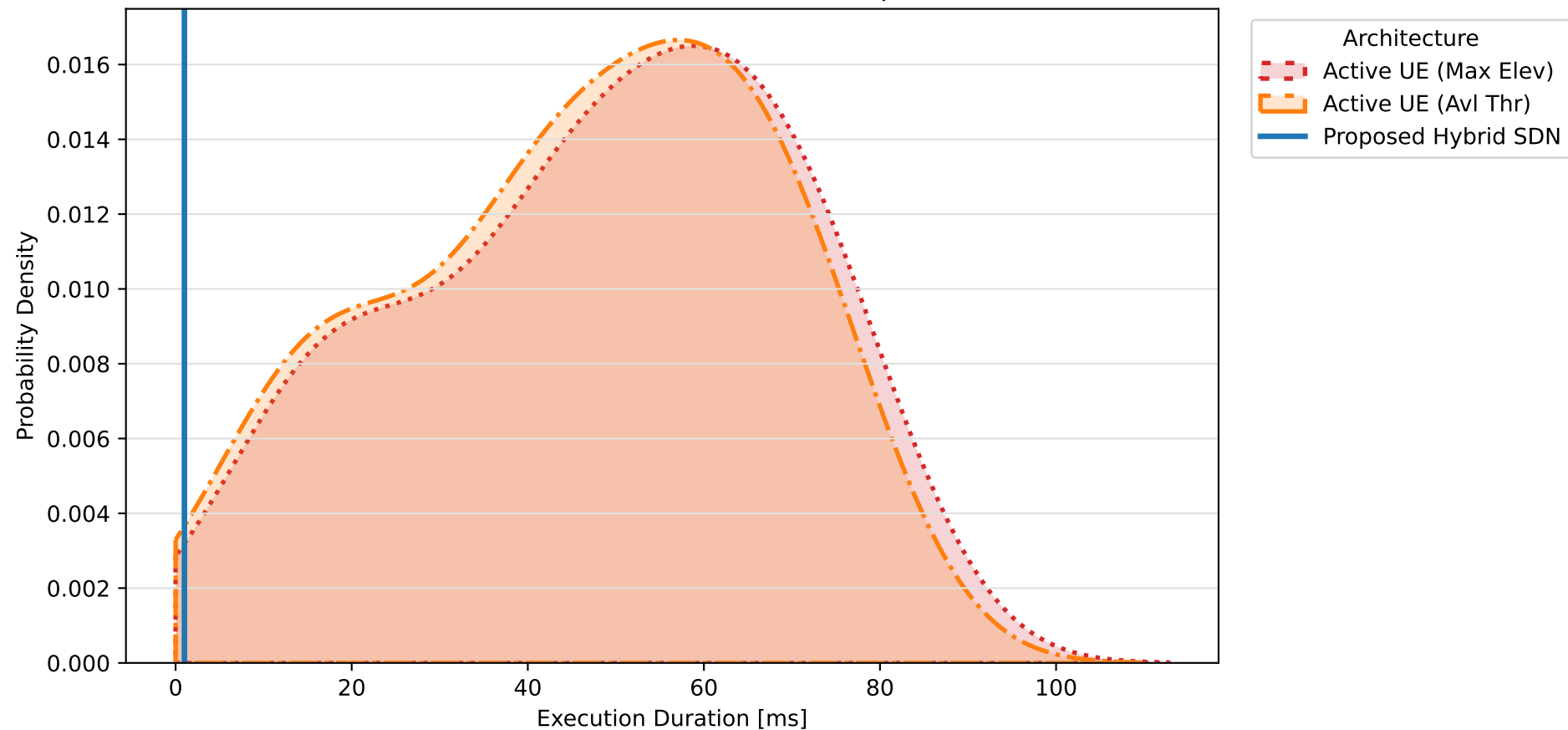
Intra-Satellite Handover Duration Comparison
