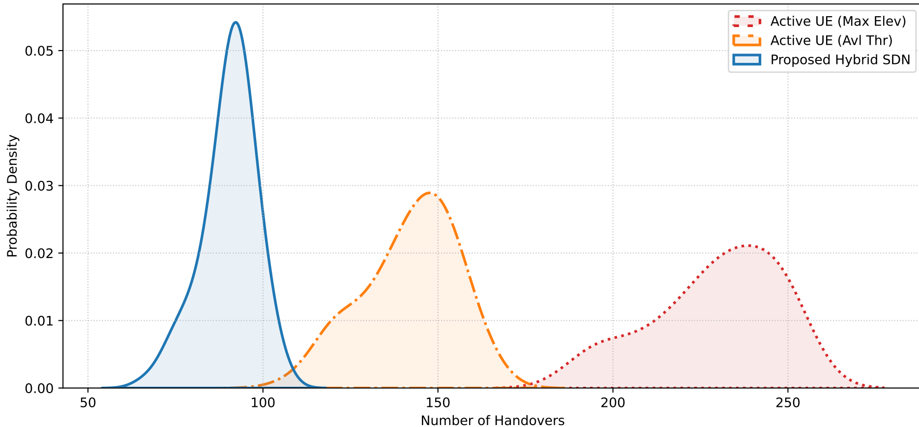
PDF of Intra-Satellite Handovers per UE - Comparative Analysis
