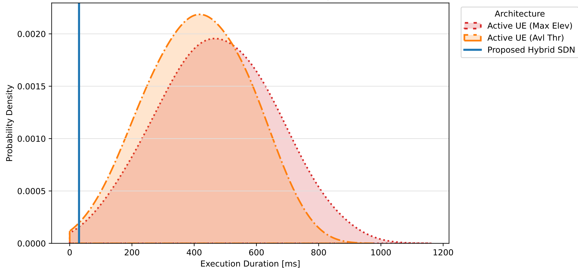
Inter-Satellite Handover Duration Comparison
