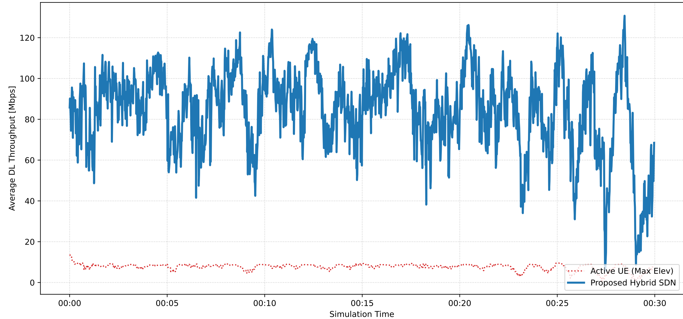
Global Average Downlink Throughput Comparison
