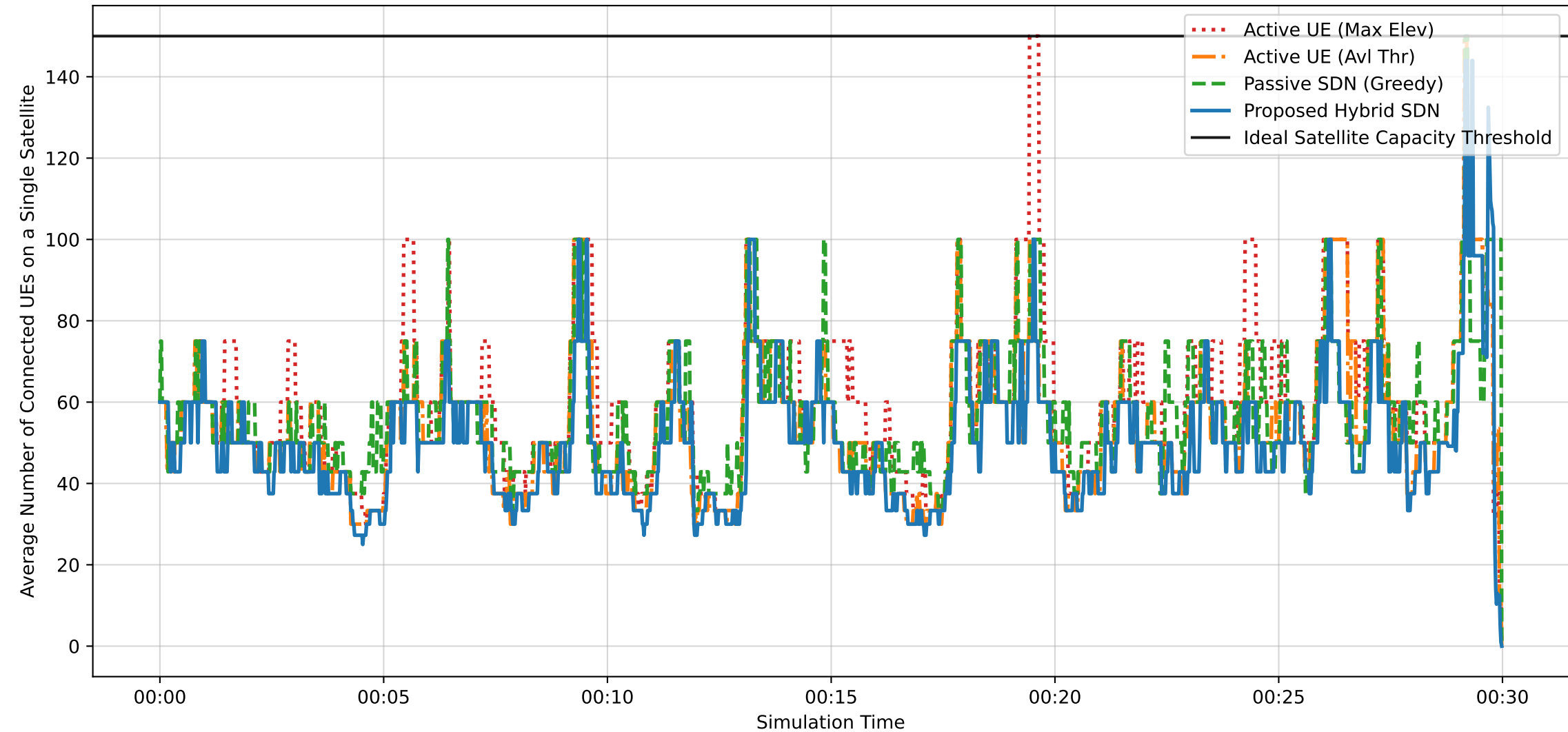
Network Congestion: Average Load per Satellite Comparison
