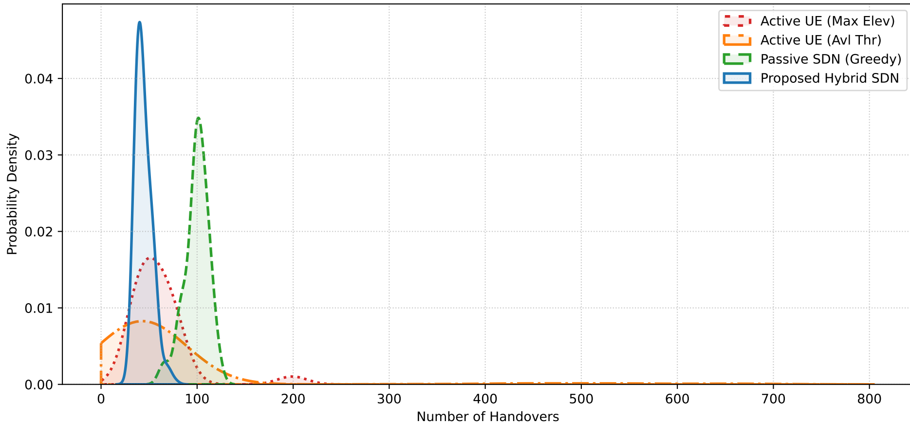
PDF of Inter-Satellite Handovers per UE
