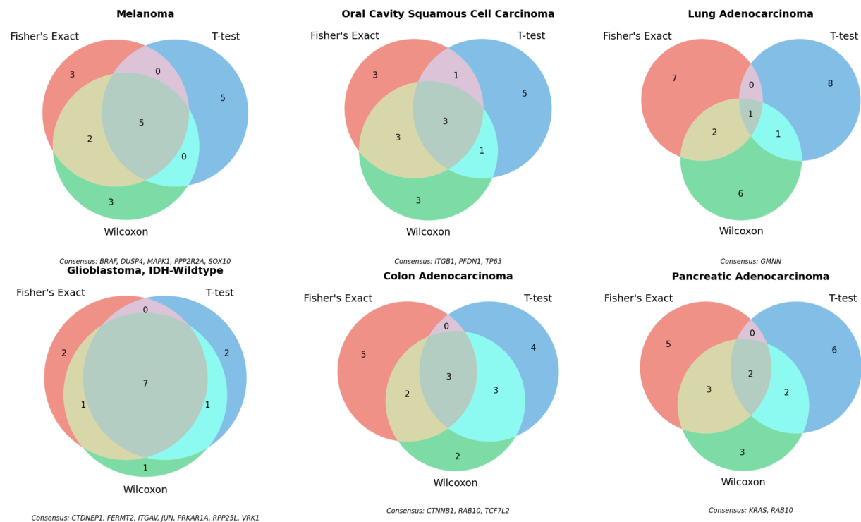
Figure S1. Pan-cancer validation of the consensus dependency framework. Venn diagrams showing the overlap of significant hits from Fisher's exact test, t-test, and Wilcoxon rank-sum test for six representative cancer indications. Consensus hits (triple intersection) recover established lineage dependencies including BRAF/MAPK1/SOX10 in melanoma, CTNNB1 in colon adenocarcinoma, and KRAS in pancreatic adenocarcinoma, validating the approach prior to application to AT/RT.
