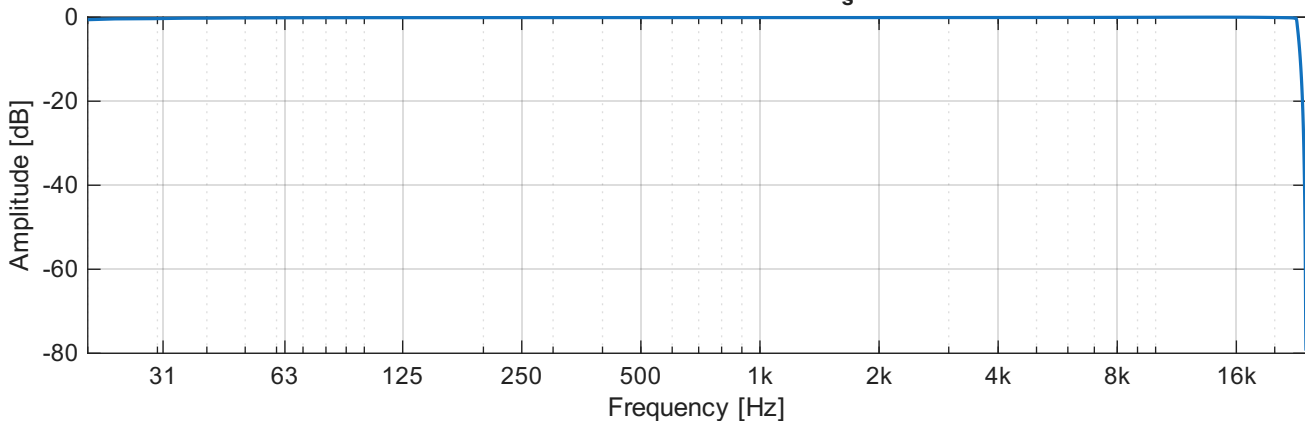
Frequency Response - REC08 s weep
