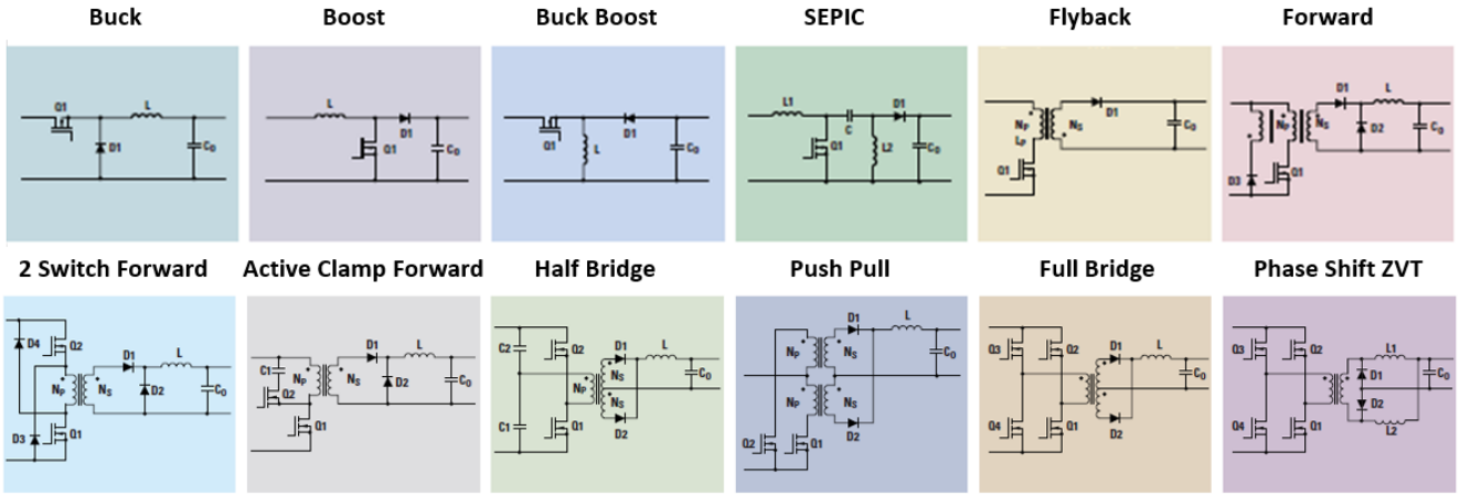
Fig. 2. Power electronics topologies and their operational principles: https://www.ti.com/lit/ml/slwu001g/slwu001g.pdf . The majority of practical power electronics converters are derived from these topologies. Each of these topologies can serve as a basis for conducting a domain-specific Turing test in power electronics. Comprehending the operational principles of these topologies constitutes the initial step towards achieving AGI in power electronics.
