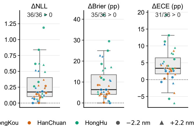
(e) Original-response probabilistic metrics
