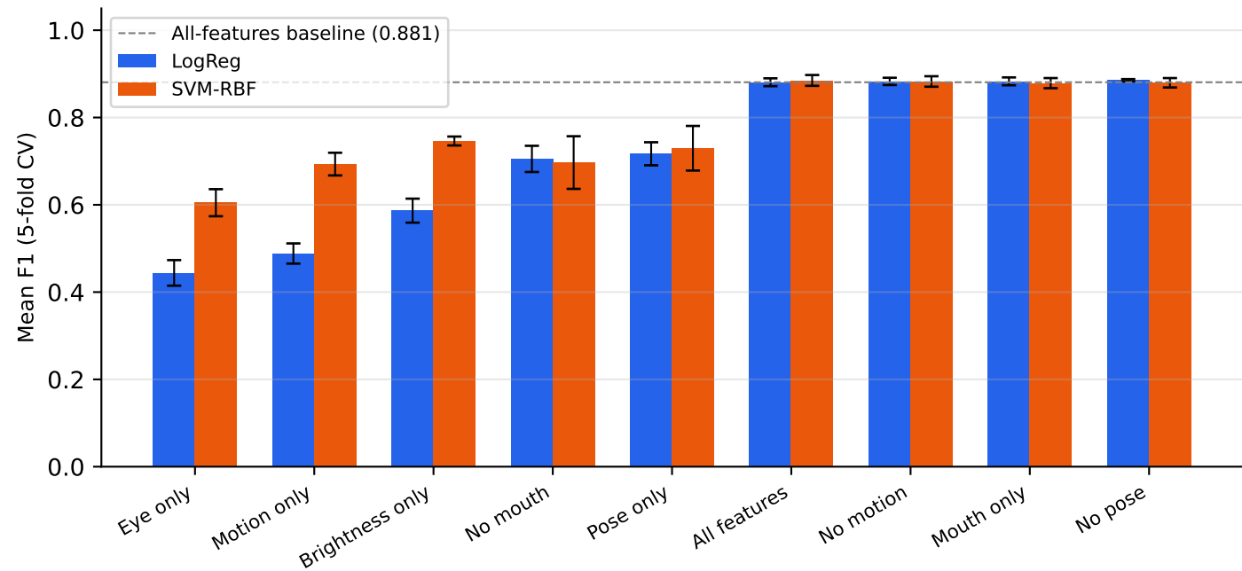
Ablation Study: F1 by Feature Subset
