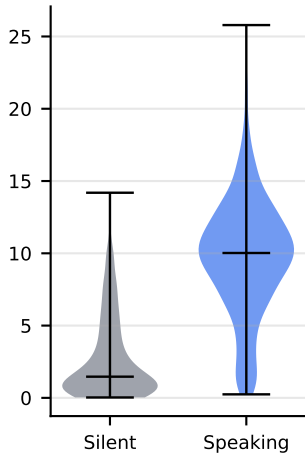
Mouth Openness
