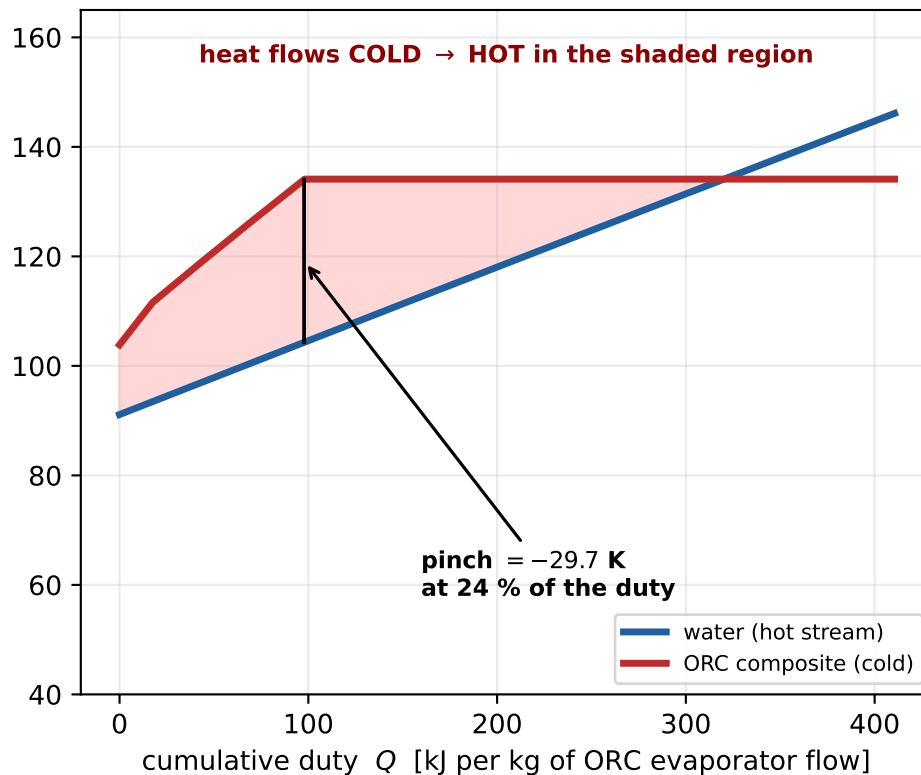
(b) v0.8 — hot-end rule, T_{3e} = 134.1 °C, \eta = 0.2320
