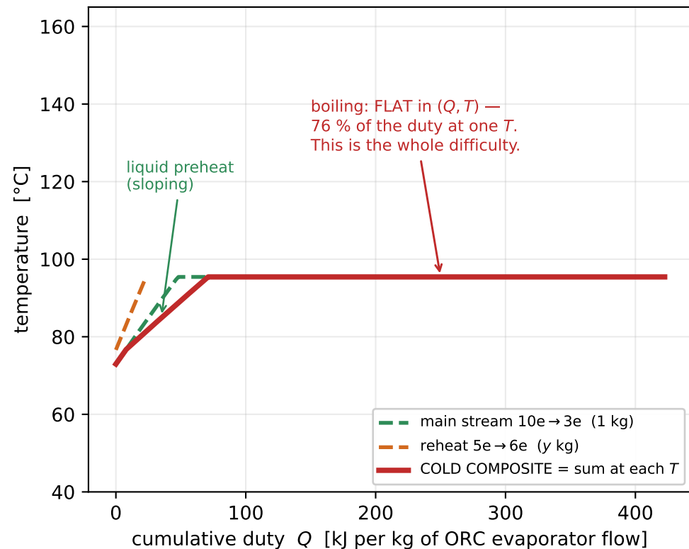
(a) building the cold composite
