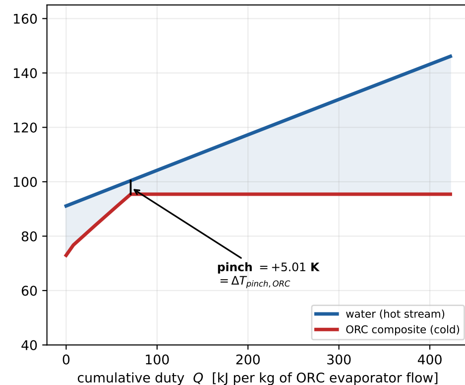
(c) v0.9 — pinch-feasible, T_{3e} = 95.4 °C, \eta = 0.1738
