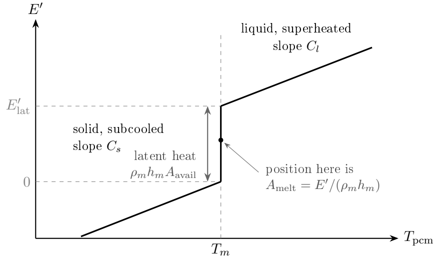
Figure 1: The enthalpy curve, Eq. (46). Reading it as E'(T) it is multivalued at T_m — which is exactly why T cannot be the state. Reading it as T(E') , the direction the code uses, it is single-valued everywhere. Position on the vertical segment is the melt fraction.
