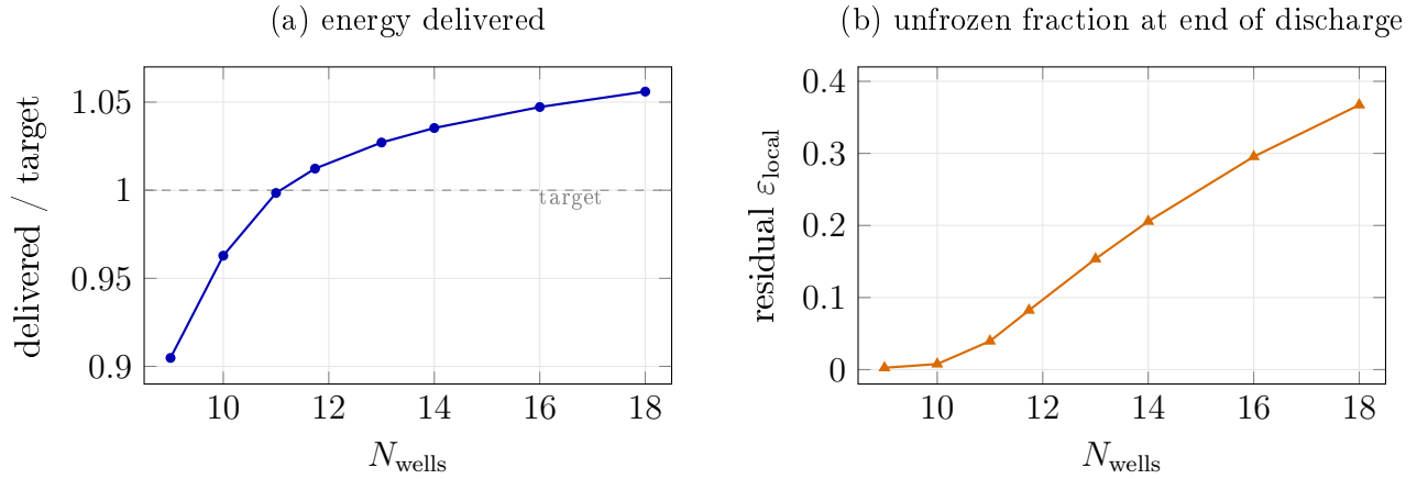
Figure 8: Cyclic steady state against exchanger count; each point is an independent march to convergence. (a) Delivered energy crosses target near N_{\text{wells}} \approx 11.0 , slightly below the latent-only count of 11.74. (b) The diagnostic: the residual melted fraction at end of discharge rises with exchanger count, because each unit is then worked less hard and proportionally less of it refreezes. An inventory-limited store would show the opposite, since a larger store would be proportionally emptier after a fixed discharge. Note that the two panels carry different quantities on similar-looking curves; they are plotted separately for that reason.
