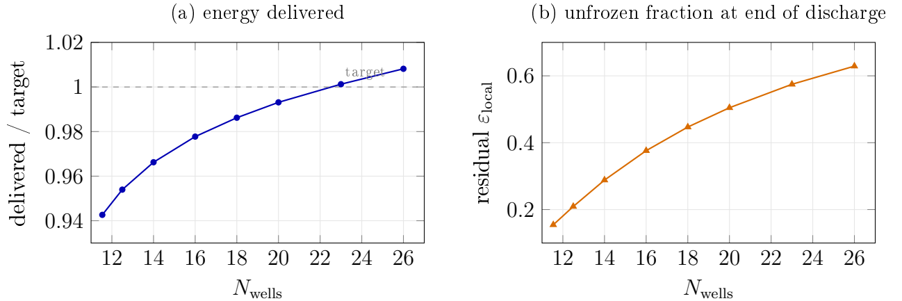
Figure 8: Cyclic steady state against exchanger count; each point is an independent march to convergence. (a) Delivered energy crosses target near N_{\text{wells}} \approx 23 , about twice the latent-only count. (b) The diagnostic: the residual melted fraction at end of discharge rises with exchanger count, because each unit is then worked less hard and proportionally less of it refreezes. An inventory-limited store would show the opposite, since a larger store would be proportionally emptier after a fixed discharge. Note that the two panels carry different quantities on similar-looking curves; they are plotted separately for that reason.
