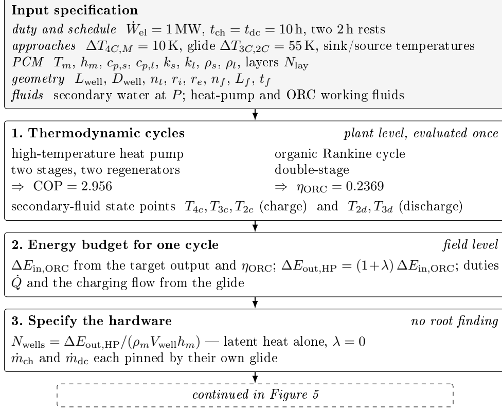
Figure 4: The solution procedure, part 1: the plant and field levels. These blocks are evaluated once, in sequence, and nothing in them is iterated. Their entire output into the rest of the calculation is five secondary-fluid state points, two flow rates and a well count — that is, a fully specified piece of hardware. The borehole model that operates it is Figure 5.
