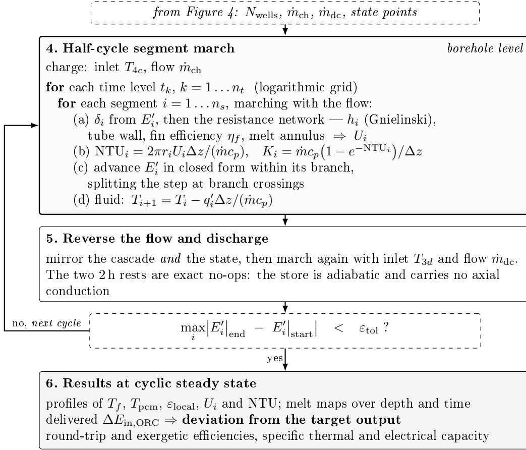
Figure 5: The solution procedure, part 2: the borehole level. Blocks 4 and 5 are the segment march of §2–§4, executed twice per cycle and repeated until the store reproduces its own initial state. This loop is the only iteration in the entire procedure: no quantity anywhere in Figures 4 and 5 is obtained by root finding, which is a consequence of Eq. (20) rather than a choice (§5.7).
