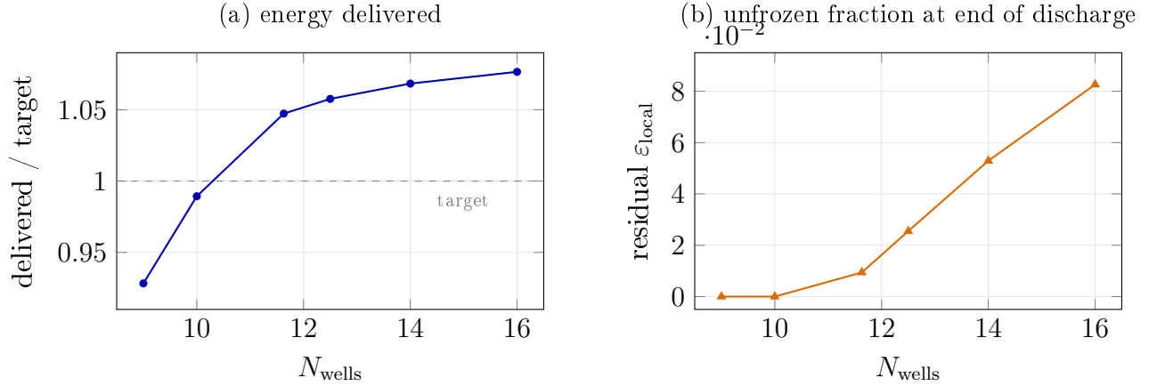
Figure 8: Cyclic steady state against exchanger count; each point is an independent march to convergence. (a) Delivered energy crosses target near N_{\text{wells}} \approx 10.1 , below the latent-only count of 11.63. (b) The diagnostic: the residual melted fraction at end of discharge rises with exchanger count, because each unit is then worked less hard and proportionally less of it refreezes. An inventory-limited store would show the opposite, since a larger store would be proportionally emptier after a fixed discharge. Note that the two panels carry different quantities on similar-looking curves; they are plotted separately for that reason.
