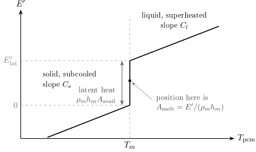
Figure 1: The enthalpy curve, Eq. (42). Reading it as E'(T) it is multivalued at T_m — which is exactly why T cannot be the state. Reading it as T(E') , the direction the code uses, it is single-valued everywhere. Position on the vertical segment is the melt fraction.
