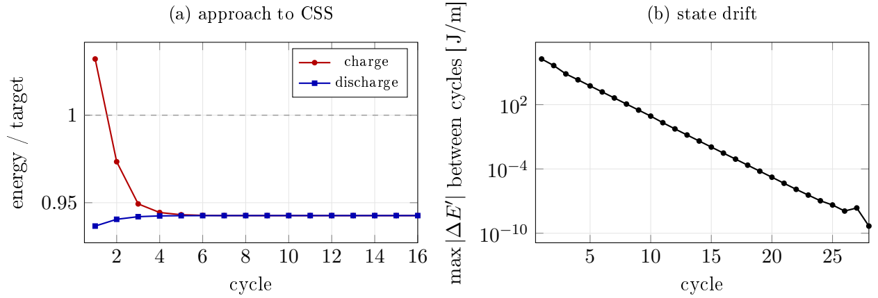
Figure 6: Convergence to cyclic steady state at the latent-only exchanger count. (a) The first cycle is the outlier: it starts from a cold, fully solid store and absorbs more than any later cycle. Charge and discharge converge to the same value, which is Eq. (20) in practice — the two curves become indistinguishable, not merely close. (b) The state drift falls geometrically; the run is stopped at 10^{-9} .
