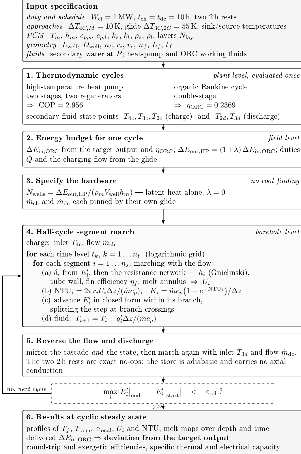
Figure 4: The solution procedure, as implemented. Blocks 1–3 are evaluated once and produce a fully specified piece of hardware; blocks 4 and 5 are the segment march of §2–§4, executed twice per cycle and repeated until the store reproduces its own initial state. The outer loop is the only iteration: nothing here is obtained by root finding, which is a consequence of Eq. (20) rather than a choice (§5.7).
