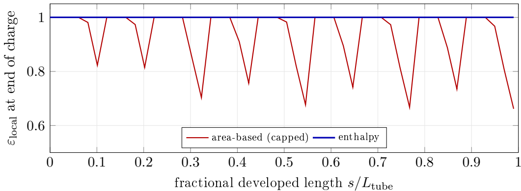
Figure 5: Local melted fraction along the exchanger at end of charge, compared at equal exchanger size with the melted fraction capped in both formulations. The sawtooth in the area-based curve is the cascade: each layer melts fully at its inlet end and incompletely at its outlet end, because a segment that has finished melting continues to draw heat at the full driving difference. Under the enthalpy formulation that segment superheats instead, its demand collapses, and the heat passes downstream — the curve is flat at unity. Spread falls from 0.405 to 0.000 (Table 5).
