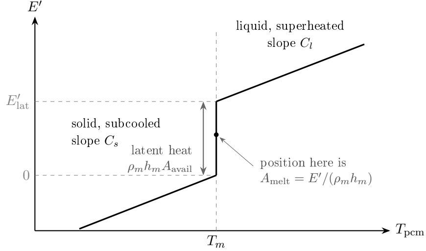
Figure 1: The enthalpy curve, Eq. (50). Reading it as E'(T) it is multivalued at T_m — which is exactly why T cannot be the state. Reading it as T(E') , the direction the code uses, it is single-valued everywhere. Position on the vertical segment is the melt fraction.
